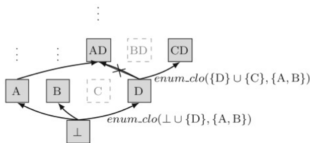
Fig. 3 Enumeration with the exclusion list
