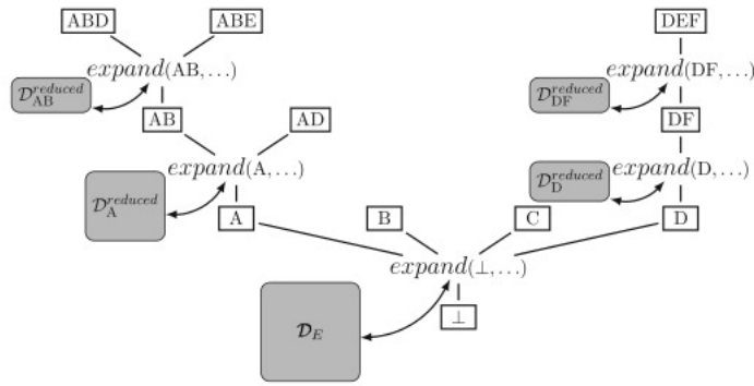
Fig. 4 The expand.l procedure explores the search space following the enumeration tree (white boxes and lines). In each call expand.l the augmentations of a closed pattern are built using the reduced dataset of this pattern (shaded boxes)
