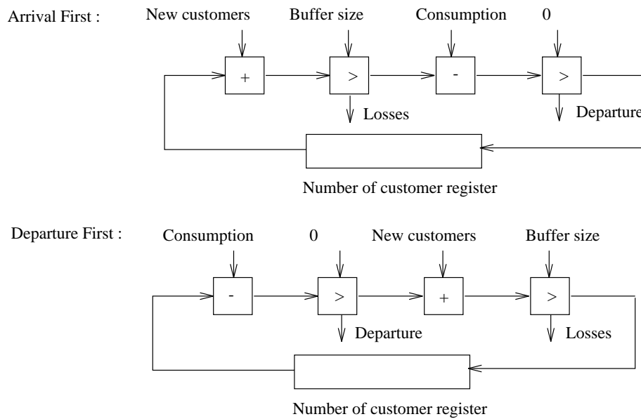
Figure 3: Hardware representation of a queue. This is a discrete time model (AF or DF) where arrival and departure processes are not fixed. In each case only a register and some logic glue are needed. Arrows give the way of propagation of integer signals.
